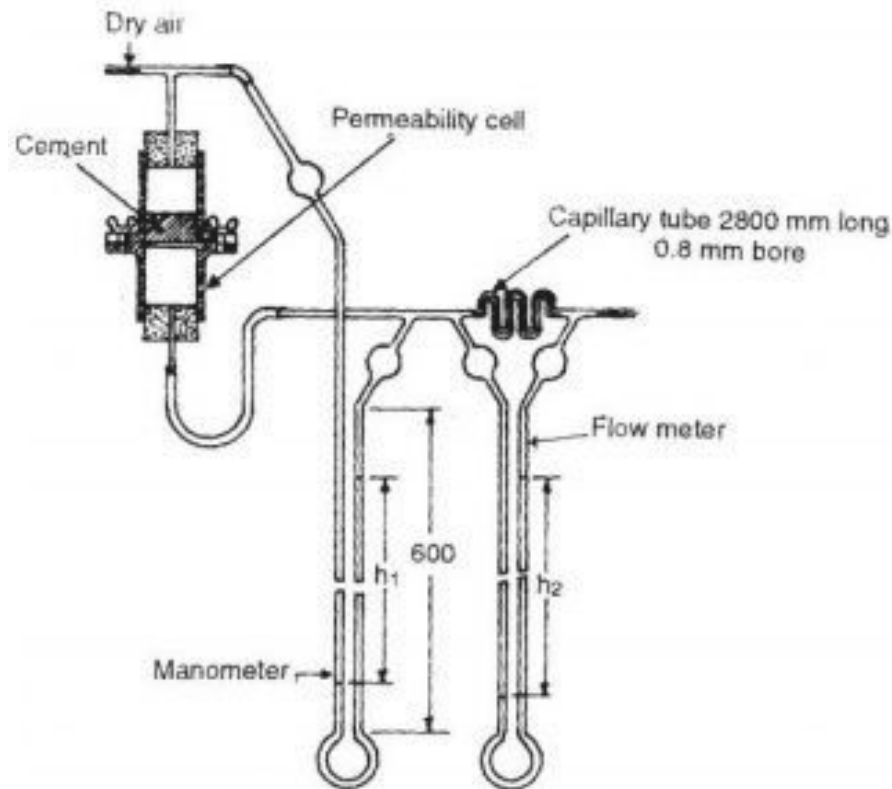
Permeability Apparatus
